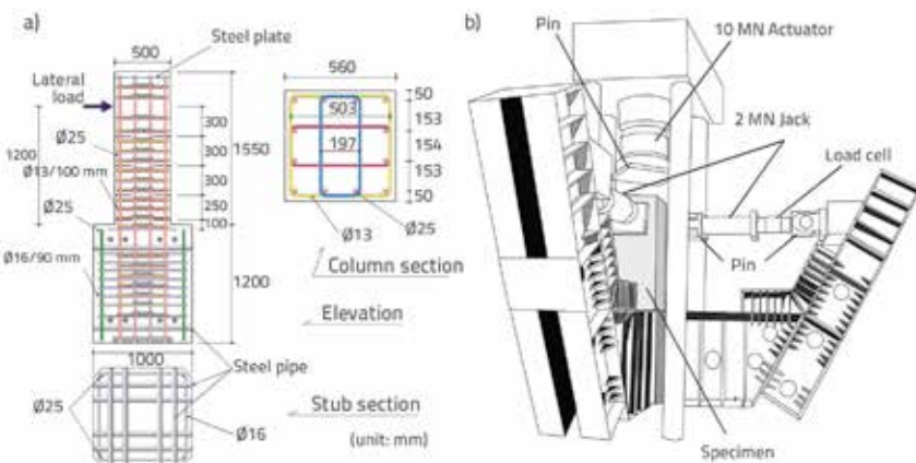
Figure 2. Specimen dimensions and loading system for large specimens [17, 18]: a) Reinforcement configurations; b) Loading system
