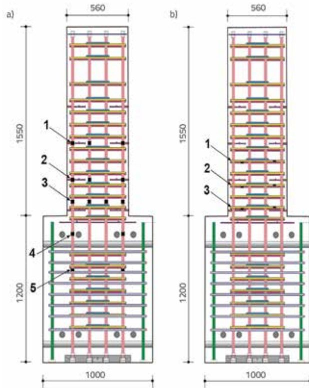
Figure 9. Position of strain gauges (layer positions) [17, 18]: a) Longitudinal reinforcement; b) transverse reinforcement
